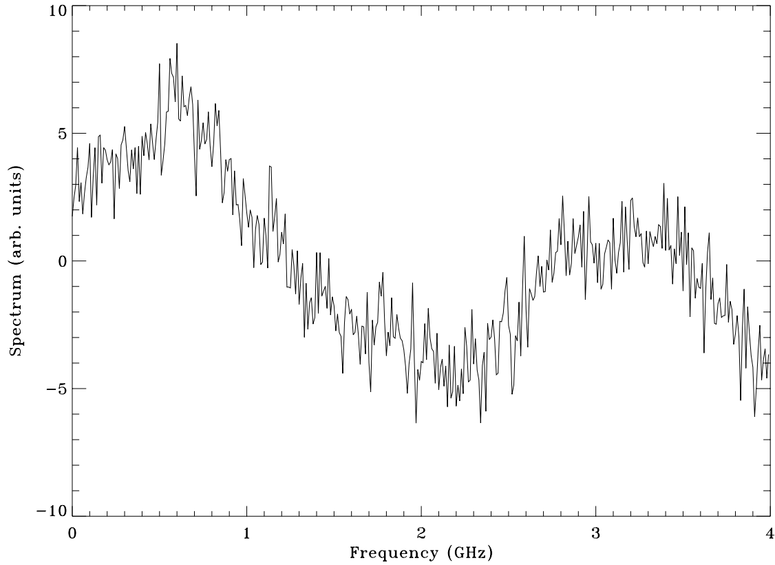
Figure 6. Sample simulated spectrum of wide bandwidth observation with a much larger 1/f gain contribution from the IF amplifier. A spectrum similar to that in the previous figure has been simulated, but now with the assumption that the chopping speed is 60 seconds. The 1/f gain fluctuation contribution is therefore larger relative to the white noise. Again, it is assumed that the IF amplifier has a correlation function described in Fig. 4. A gain fluctuation level consistent with the measurements described earlier was used. Structure in the spectrum that results from gain fluctuations is now readily apparent. A baseline offset of 6.6 units has been subtracted.
