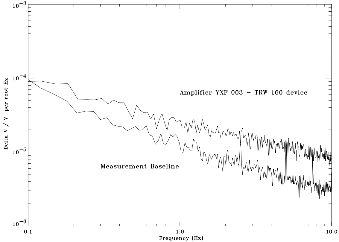
Figure 2. Measurement of amplifier gain fluctuations. The upper curve is the fluctuation level for a two-stage amplifier built with a TRW 160 micron gate width device for the first stage and a Fujitsu 200 micron gate width device for the second stage. The lower curve is the measurement baseline established with no device under test.
