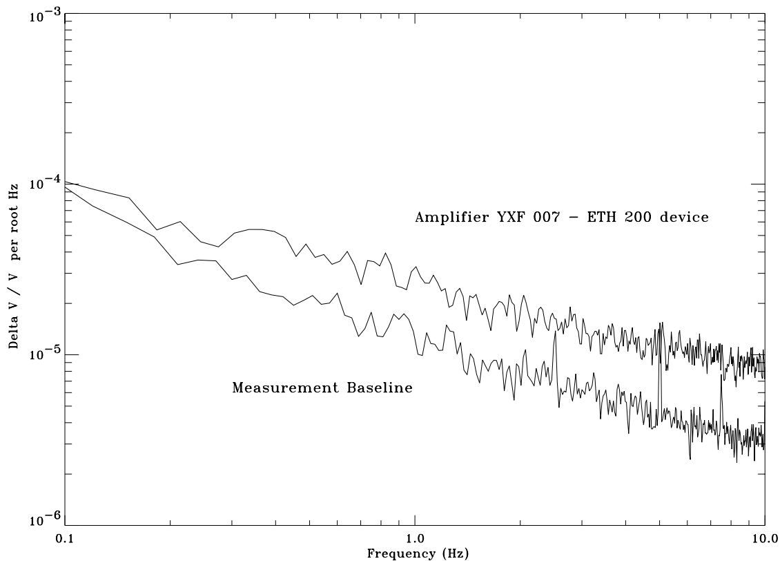
Figure 3. Measurement of amplifier gain fluctuations. The upper curve is the fluctuation level for a two-stage amplifier built with a ETH 200 micron gate width device for the first stage and a Fujitsu 200 micron gate width device for the second stage. The lower curve is the measurement baseline established with no device under test.
