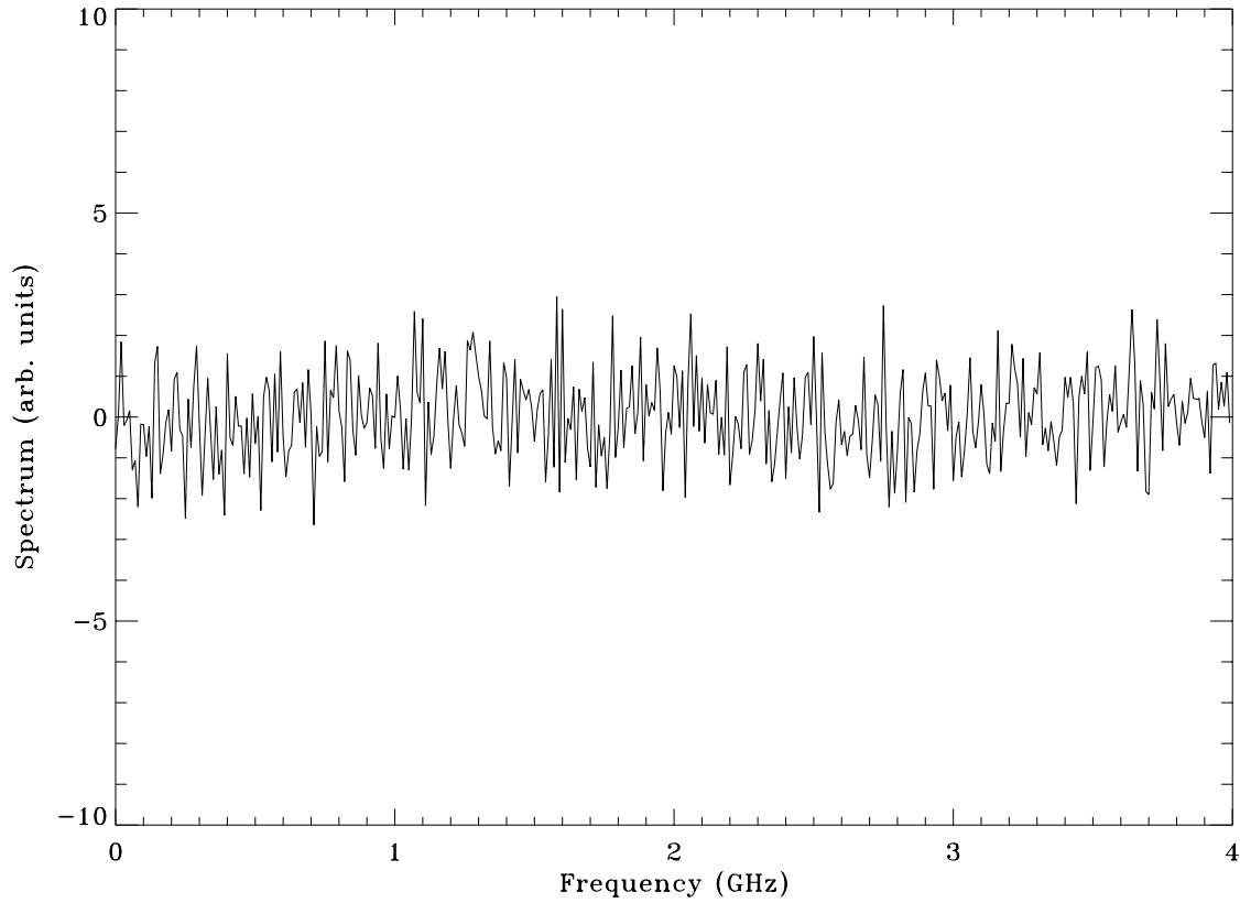
Figure 5. Sample simulated spectrum of wide bandwidth observation with 1/f gain fluctuation contribution from the IF amplifier. A spectrum has been simulated assuming that there is no source signal and that the gain fluctuation noise from the IF amplifier has a correlation function described in Fig. 4. There is little resulting structure in the spectrum due to these gain fluctuations. A gain fluctuation level consistent with the measurements described earlier was used. A chopping speed of 1 Hz has been assumed. The simulation was performed with a 10 MHz spectral bin size and 400 spectral bins.
