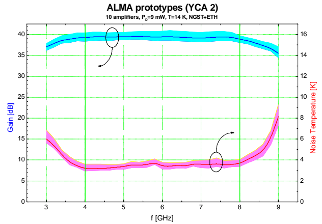
Figure 2 Cryogenic noise and gain plots of 10 ALMA amplifiers, in the same fashion as Figure 1.
