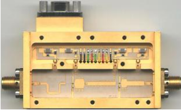
Figure 3 2-stages 4-8 GHz HIFI cryogenic LNA Development Model (DM) YCF 6. Amplifier size is 58×32×15 mm.
