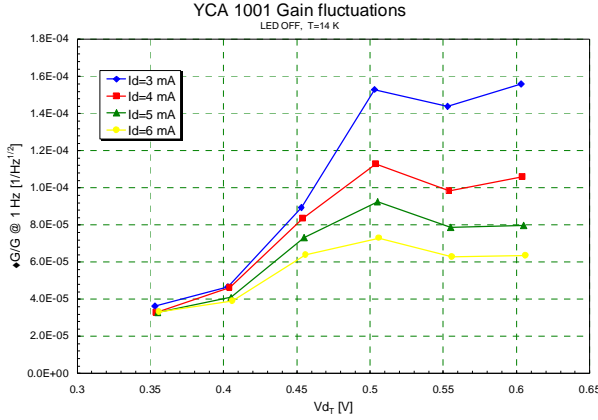
Figure 5 Measurements of the cryogenic normalized gain fluctuations (b parameter) response of a 3-stages 4-8 GHz amplifier to changes in the bias point of the 1 st stage. There is an InP device in the 1 st stage and two GaAs transistors in the 2 nd and 3 rd . This variation of bias produces only minor modifications of the noise performance.
