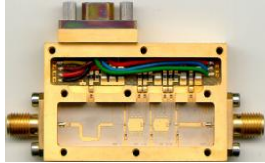
Figure 4 3-stages 4-8 GHz cryogenic LNA prototype for ALMA band 7. Amplifier size is 46×29×9 mm.
