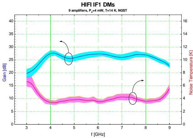
Figure 1 Cryogenic noise and gain plots of 9 DMs built for HIFI. The colored bands are defined by worst and best values for all the amplifiers. The solid line is the average of the series.
