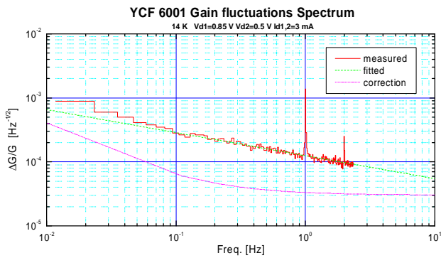
Figure 2 Example of calibrated measurement of the Spectral Density of Normalized Gain Fluctuations of amplifier YCF 6001. The measured data presented has been corrected to eliminate the contribution of system fluctuations. The value of the correction is also shown in the graph as a reference. The peak appearing at 1 Hz is due to the cycle of CTI 1020 refrigerator. A smaller peak at 2 Hz is also visible.
