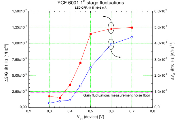
Figure 6 Measurements of the variation with drain voltage of fluctuations in gain and gate voltage in the 1 st stage of a HIFI-DM. A correlation is apparent. The values of gain stability for the lower drain voltages are contaminated by system noise.
