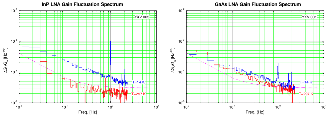
Figure 4 Gain fluctuations spectra for two identical amplifiers with InP and GaAs devices respectively. The room temperature spectrum of the InP amplifier lies below the calibration spectrum of the normalized gain fluctuations of the measurement system. The lines appearing at 1 and 2 Hz are due to the refrigerator cycle, and the one at 1.7 Hz is probably related with mechanical vibrations of the vacuum pump.
