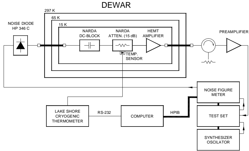
Figure 1 Block diagram of cryogenic noise measurements with the cold attenuator method.
